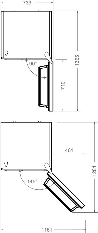
TOP VIEW
